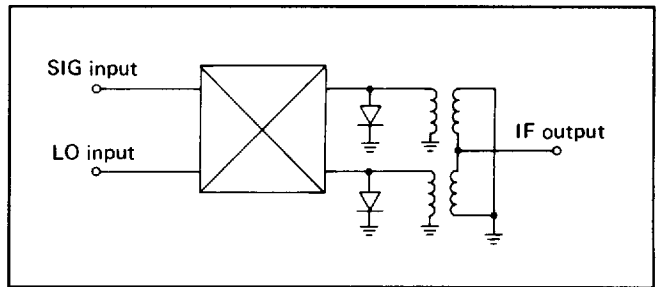
Figure 3. Balanced Mixer Using Diode Pairs With Suffix "M"
