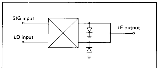
Figure 4. Balanced Mixer Using Diode Pairs With Suffix "MR"
