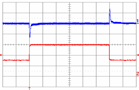
Fig. 21: Output voltage response to load current step-change (7.5 A – 15 A – 7.5 A) at V_{in} = 48\text{ V} . Top trace: output voltage (100 mV/div). Bottom trace: load current (5 A/div.). Current slew rate: 5 A/ \mu\text{s} . C_o = 450\ \mu\text{F} tantalum + 1 \mu\text{F} ceramic. Time scale: 0.2 ms/div.
