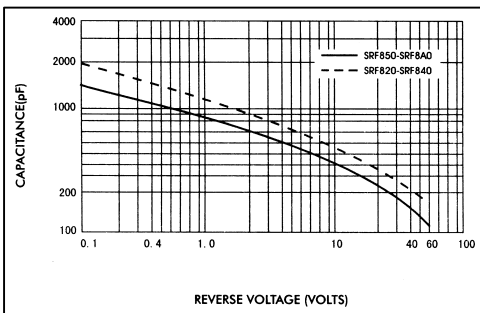
FIG.4-TYPICAL JUNCTION CAPACITANCE
