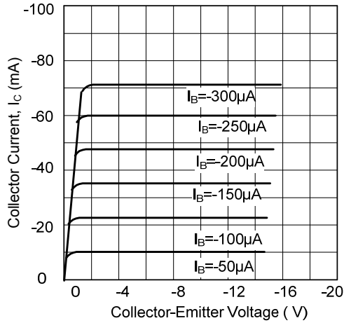
Fig.1 Static Characteristics
