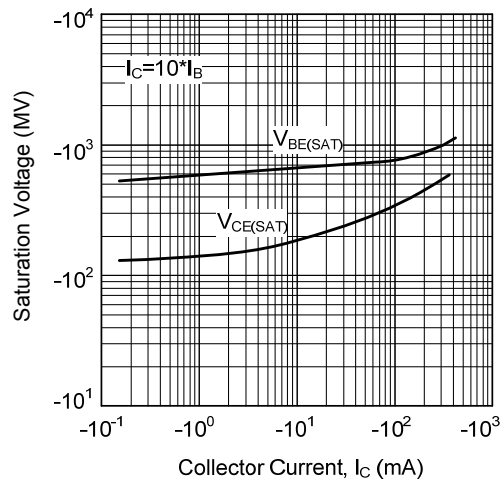
Fig.4 Saturation Voltage
