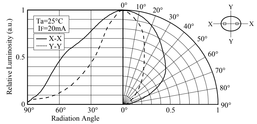
■ Directivity (NSPG346BS)
