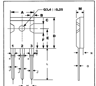
TO-247 (3P)
