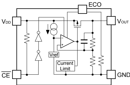
R1161xxxxA (CE pin "L" active)
