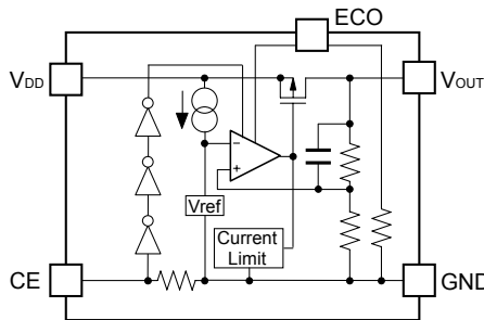
R1161xxxxB (CE pin "H" active)
