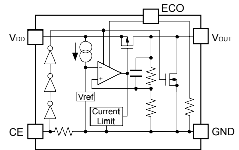
R1161xxxxD (With Auto-Discharge function)
