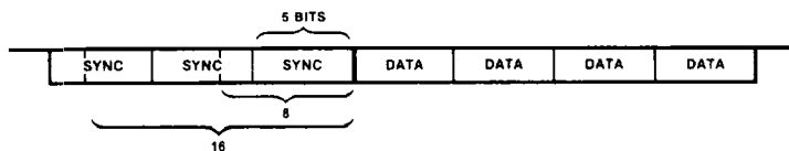
Figure 10. Data Communication
