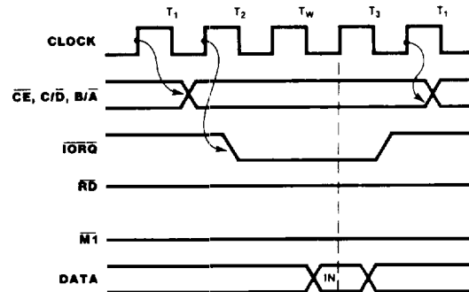
Figure 16. Write Cycle
