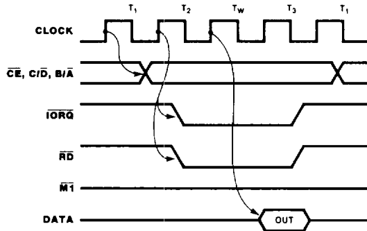
Figure 15. Read Cycle
