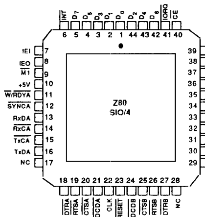
Figure 7a. 44-pin Chip Carrier, Pin Assignments
