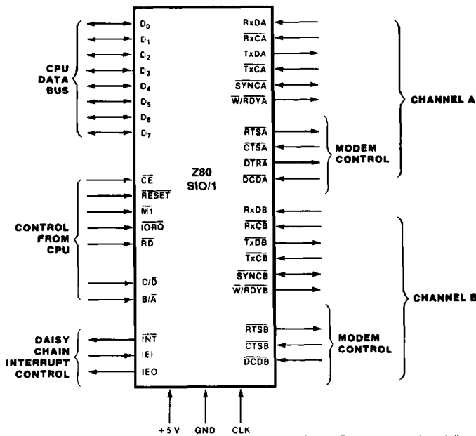
Figure 3. Pin Functions
