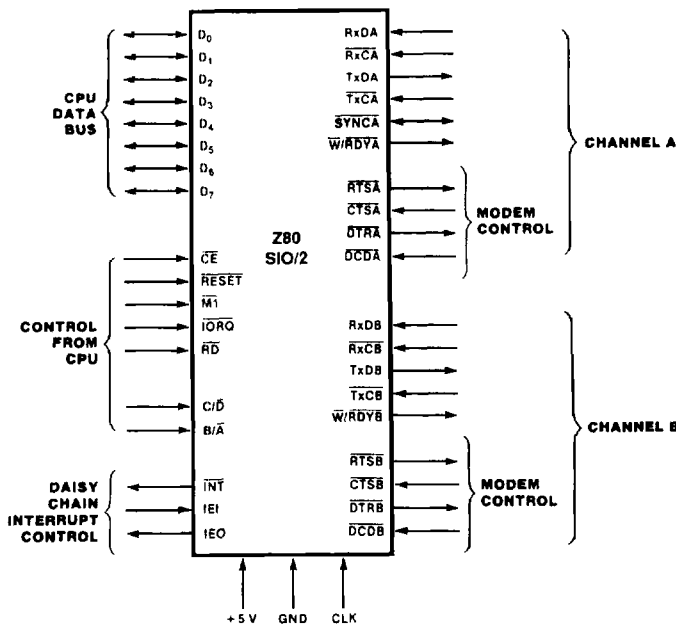
Figure 1. Pin Functions
