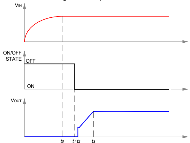
Fig. 7: Start-up scenario #2.
