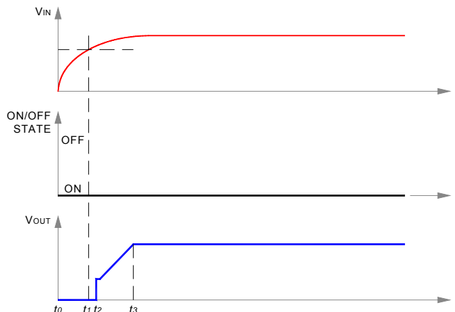
Fig. 6: Start-up scenario #1.
