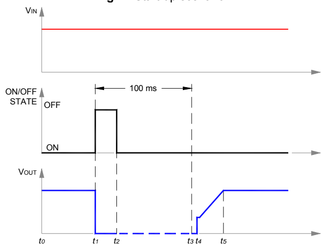
Fig. 8: Start-up scenario #3.
