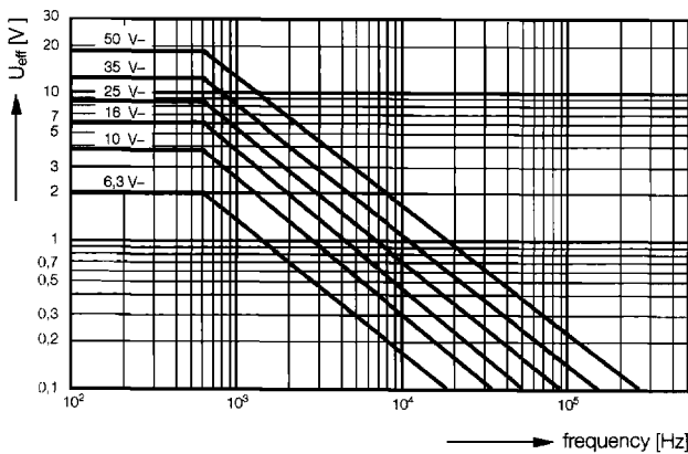
Diagram 17: Permissible superimposed AC voltage versus rated voltage and frequency at +20°C ETQW 3
