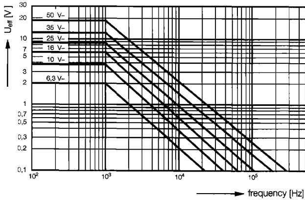
Diagram 16: Permissible superimposed AC voltage versus rated voltage and frequency at +20°C ETQW 2
