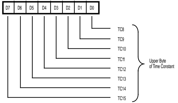
Read Register 13
