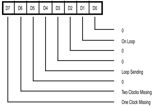
Read Register 10
