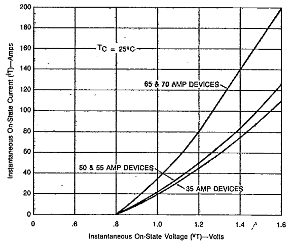
FIGURE 6B — Instantaneous On-State Current vs On-State Voltage (Typical)
