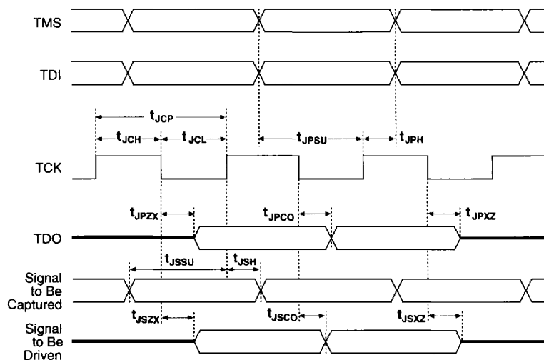
Figure 32. APEX 20K JTAG Waveforms
