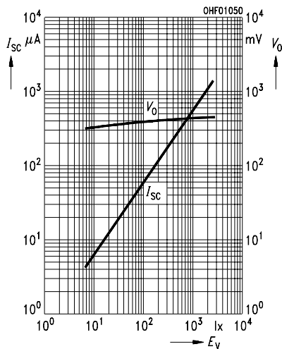
Short-circuit current I_{SC} = f(E_v)
