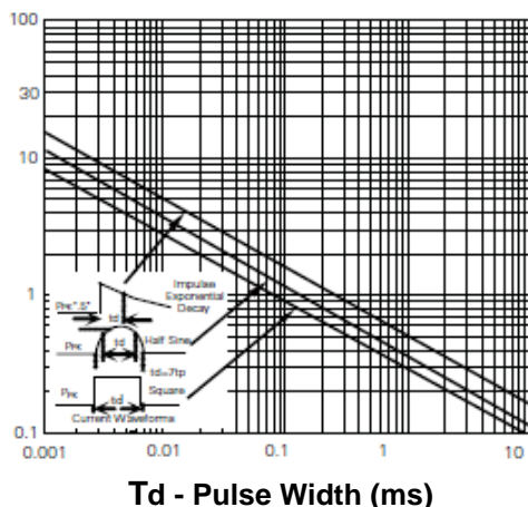
Fig.1- Peak Pulse Power Rating Curve
