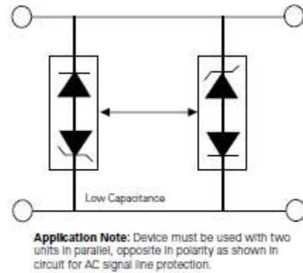
Fig.4- AC Line Protection Application
