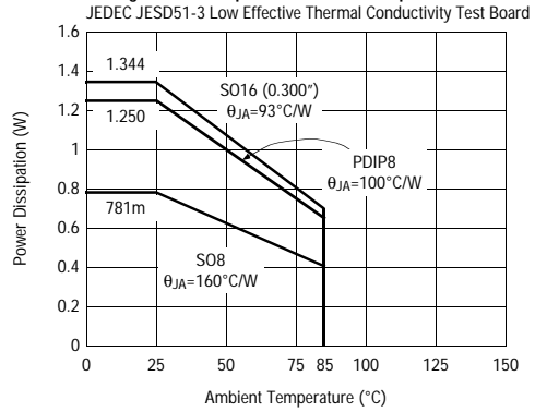
Package Power Dissipation vs Ambient Temp.
