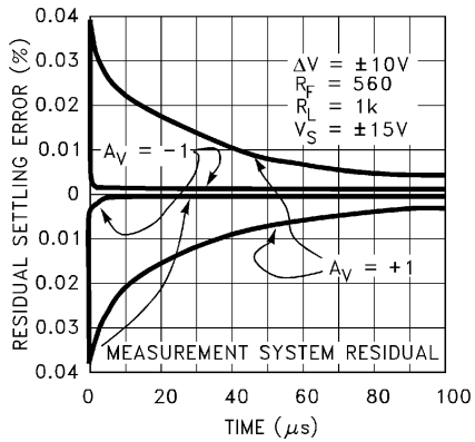
Long Term Settling Error
