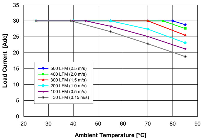
Fig. 1: Available load current vs. ambient air temperature and air flow rates for Q24T30020 converter mounted vertically with air flowing from pin 3 to pin 1, MOSFET temperature \leq 120^{\circ}\text{C} , V_{in} = 27\text{ V} .
