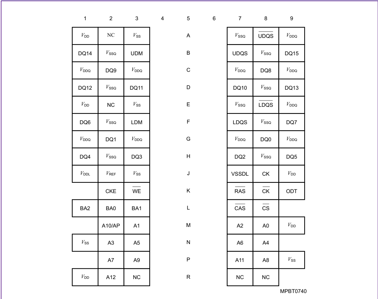
FIGURE 2 Chip Configuration for x16 Components in FBGA-84, Top View
