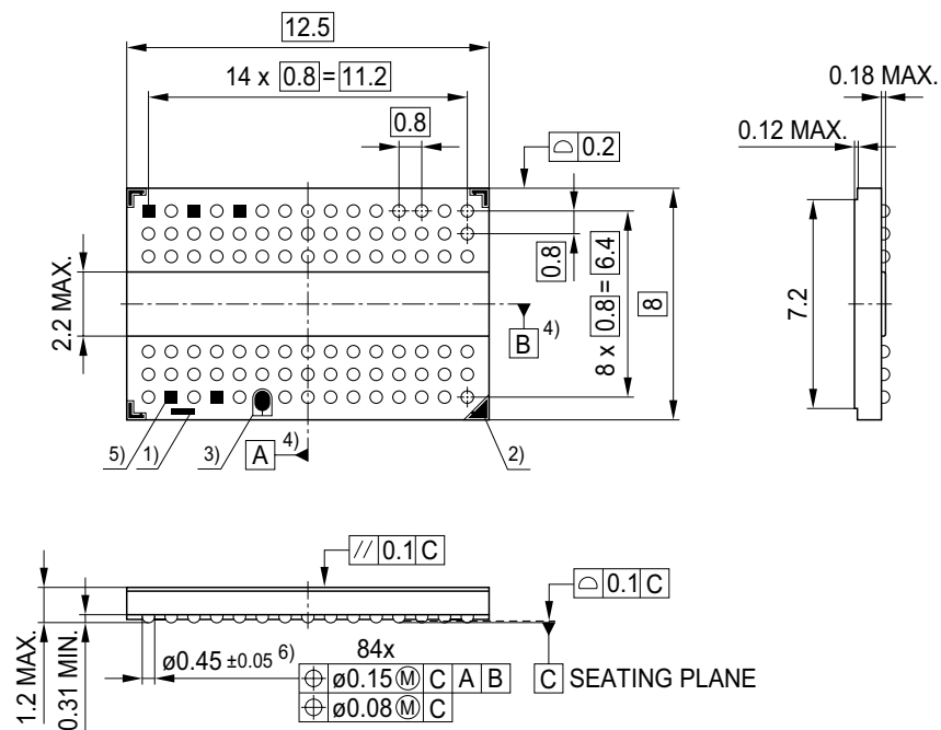
FIGURE 11 Package Outline PG-TFBGA-84
