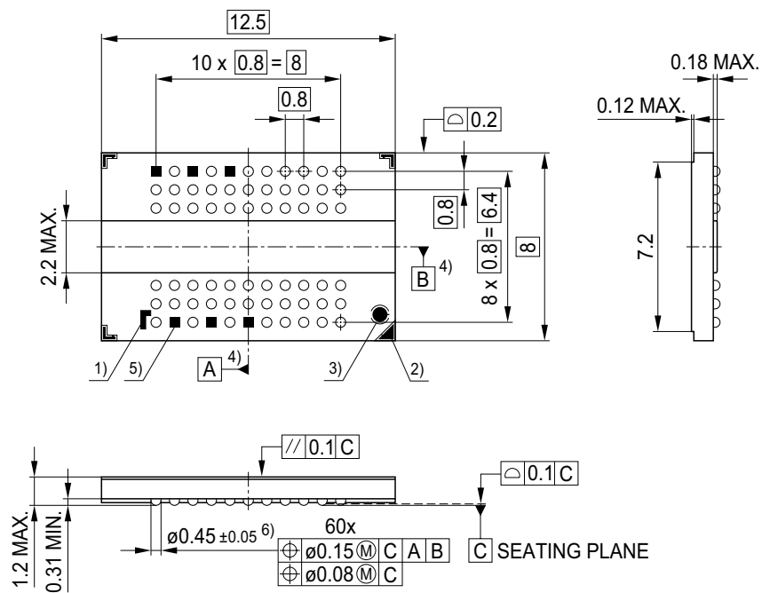
FIGURE 10 Package Outline PG-TFBGA-60
