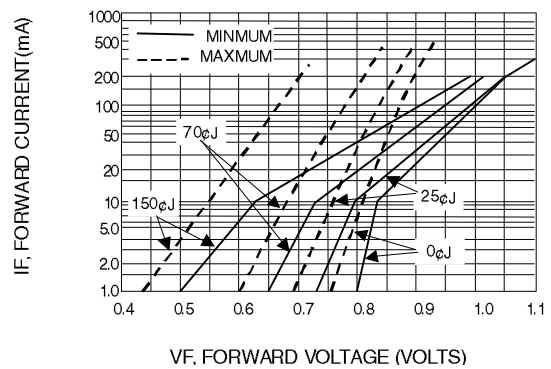
Fig. 10-TYPICAL FORWARD CHARACTERISTICS
