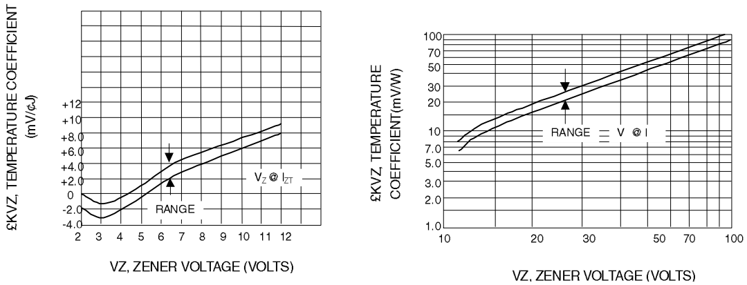
Fig. 2-TEMPERATURE COEFFICIENTS (-55 \phi J TO +150 \phi J TEMPERATURE RANGE; 90% OF THE UNITS ARE IN THE RANGES INDICATED.)
