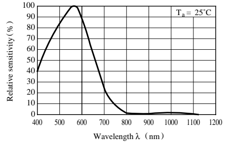
Fig. 4 Spectral Sensitivity
