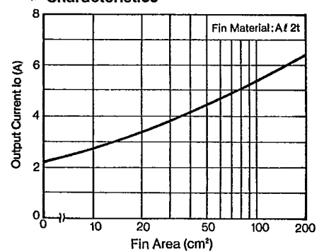
I o - Fin Characteristics
