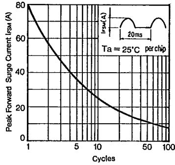
I FSM Characteristics
