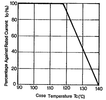
I F(AV) - T c Derating
