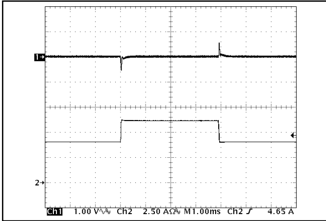
Figure 7: Output voltage response to step-change in load current (50%-75%-50% of I_{out(max)} ; dI/dt = 0.1 A/\mu s ). Load cap: 1 \mu F ceramic and 15 \mu F tantalum capacitors. Ch 1: V_{out} (1 V/div), Ch 2: I_{out} (2.5 A/div).
