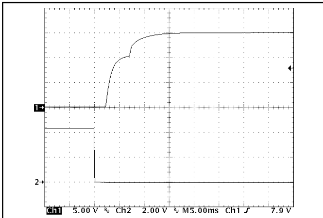
Figure 9: Turn-on transient at full load (resistive load) (5 ms/div). Input voltage pre-applied. Ch 1: V_{out} (5 V/div), Ch 2: ON/OFF input (2 V/div).
