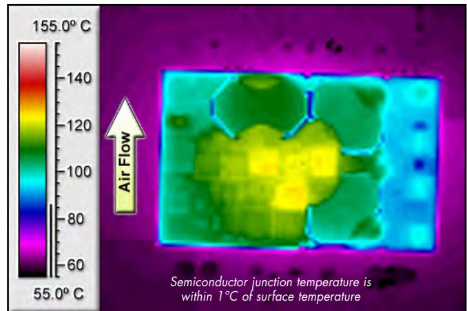
Figure 4: Open frame converter thermal plot at 7.9 amp load current (118.5 W) with 55°C air flowing at the rate of 200 LFM. Air flows across the converter from pin 3 to pin 1 (nominal input voltage).
