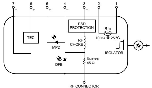
Figure 1. D1861A DML Electrical Schematic
