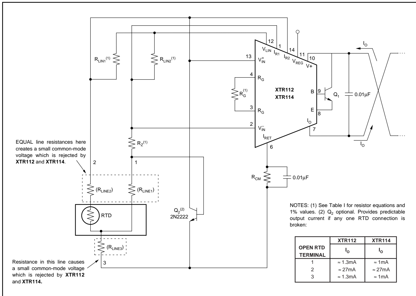
FIGURE 3. Three-Wire Connection for Remotely Located RTDs.
