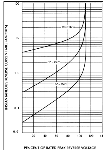
FIG.3-TYPICAL REVERSE CHARACTERISTICS
