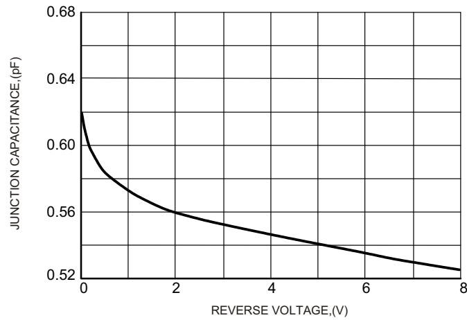
FIG.3-TYPICAL JUNCTION CAPACITANCE
