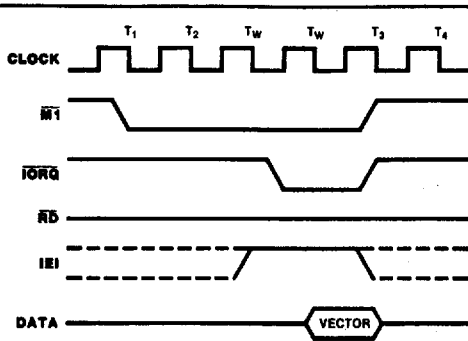
Figure 7. Interrupt Acknowledge Cycle
