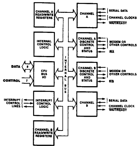
Figure 3. Block Diagram
