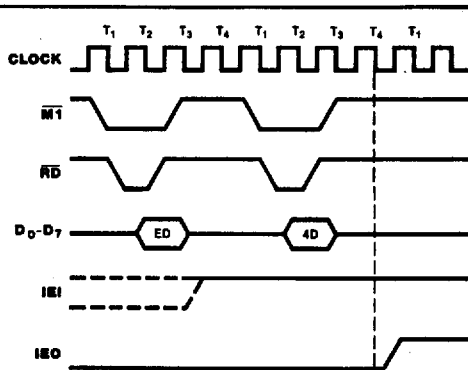
Figure 8. Return from Interrupt Cycle
