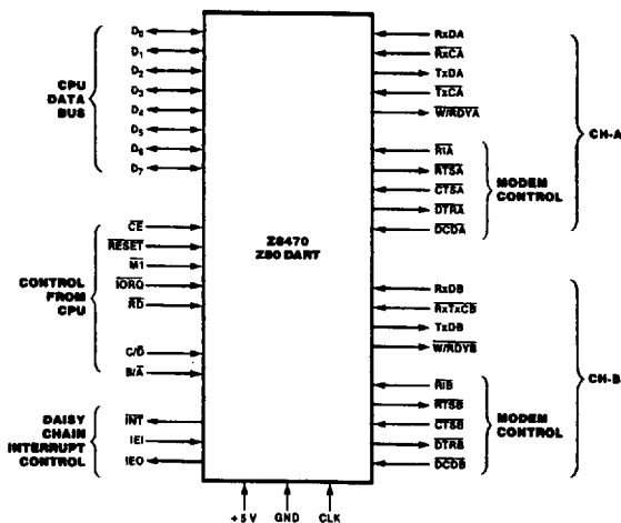
Figure 1. Pin Functions
