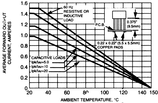
FIG.1-DERATING CURVE
