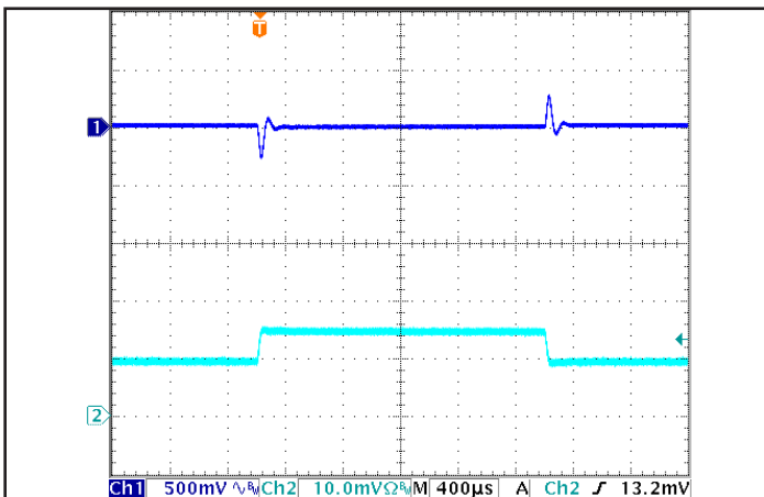
Figure 5: Output voltage response to step-change in load current (50% -75% -50% of I out (max); dI/dt = 0.1 A/μs). Load cap: 100 μF electrolytic capacitor. Ch 1: V out (500 mV/div), Ch 2: I out (5 A/div)
