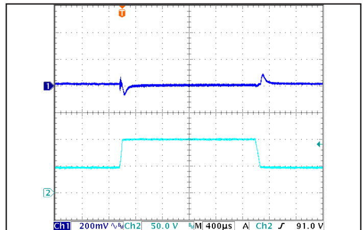
Figure 6: Output voltage response to step-change in input voltage (1000 V/ms). Load cap: 100 \mu F , electrolytic output capacitance. Ch 1: V_{out} (200 mV/div), Ch 2: V_{in} (50 V/div).
