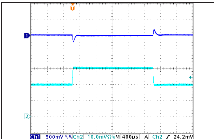
Figure 5: Output voltage response to step-change in load current (50% -75% -50% of Iout(max); dI/dt = 0.1 A/μs). Load cap: 100 μF electrolytic capacitor. Ch 1: Vout (500 mV/div), Ch 2: Iout (1 A/div).
