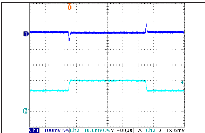
Figure 5: Output voltage response to step-change in load current (50% -75% -50% of I out (max); dI/dt = 0.1 A/μs). Load cap: 100 μF electrolytic capacitor. Ch 1: V out (100 mV/div), Ch 2: I out (10 A/div).
