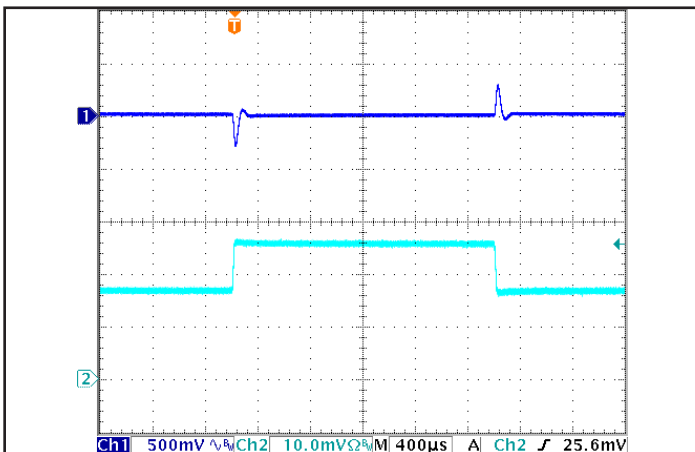
Figure 5: Output voltage response to step-change in load current (50% -75% -50% of I_{out(max)} ; dI/dt = 0.1 A/\mu s ). Load cap: 100 \mu F electrolytic capacitor. Ch 1: V_{out} (500 mV/div), Ch 2: I_{out} (2 A/div)
