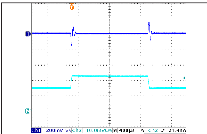
Figure 5: Output voltage response to step-change in load current (50% -75% -50% of I out (max); dI/dt = 0.1 A/μs). Load cap: 100 μF electrolytic capacitor. Ch 1: V out (200 mV/div), Ch 2: I out (5 A/div).
