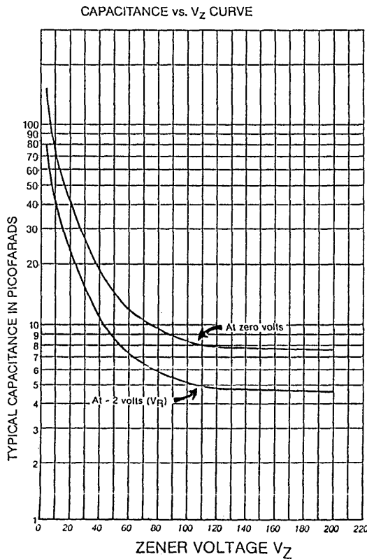
FIGURE 3 CAPACITANCE vs. ZENER VOLTAGE (TYPICAL)
