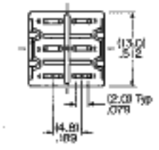
M2011 & M2021 models do not have terminals 1 & 4.
