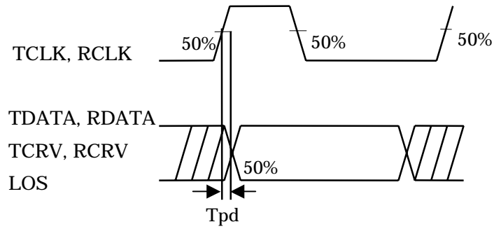
Fig.8 Transmitter Timing
