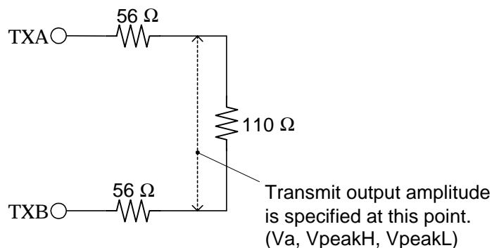
Fig.1 Measurement circuit
