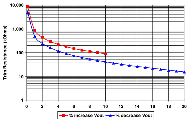
Figure C: Trim Graph for 2.5Vout module
