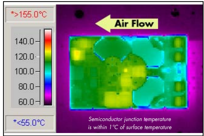
Figure 8: Thermal plot of converter at 24 amp load current with 55°C air flowing at the rate of 200 LFM. Air is flowing across the converter from output to input (nominal input voltage).
