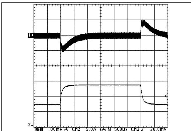
Figure 11: Output voltage response to step-change in load current (50%-75%-50% of I_{out(max)} ; dI/dt = 0.1A/\mu s ). Load cap: 10 μF, 100 mΩ ESR tantalum cap and 1 μF ceramic cap. Ch 1: Vout (100mV/div), Ch 2: Iout (5A/div).
