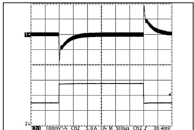
Figure 12: Output voltage response to step-change in load current (50%-75%-50% of I_{out(max)} ; dI/dt = 5A/\mu s ). Load cap: 470 μF, 30 mΩ ESR tantalum cap and 1 μF ceramic cap. Ch 1: Vout (100mV/div), Ch 2: Iout (5A/div).
