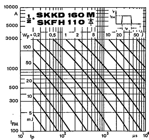
Fig. 15 b Forward energy dissipation, rectangular
