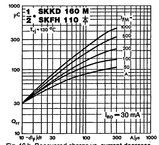
Fig. 16 b Recovered charge vs. current decrease
