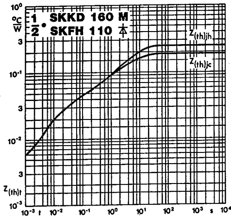
Fig. 18 b Transient thermal impedance vs. time
