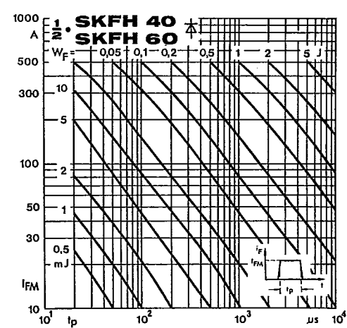
Fig. 15 a Forward energy dissipation, rectangular
