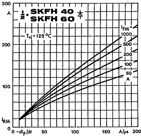
Fig. 17 a Peak recovery current vs. current decrease
