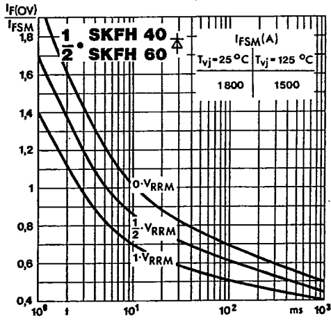
Fig. 20 a Surge overload current vs. time
