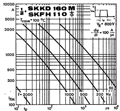
Fig. 14 f Rated rectangular peak forward current
