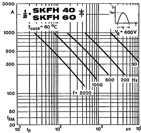
Fig. 12 a Rated sinusoidal peak forward current
