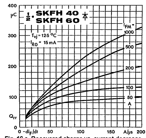
Fig. 16 a Recovered charge vs. current decrease
