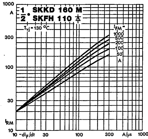
Fig. 17 b Peak recovery current vs. current decrease
