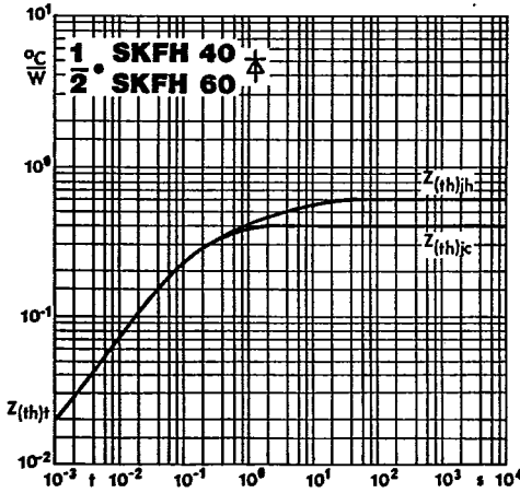
Fig. 18 a Transient thermal impedance vs. time
