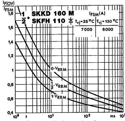
Fig. 20 b Surge overload current vs. time
