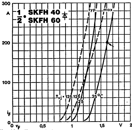
Fig. 19 a Forward characteristics
