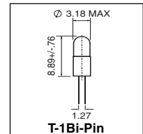
T-1 Bi-Pin
