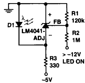
Figure 4. Voltage Level Detector
