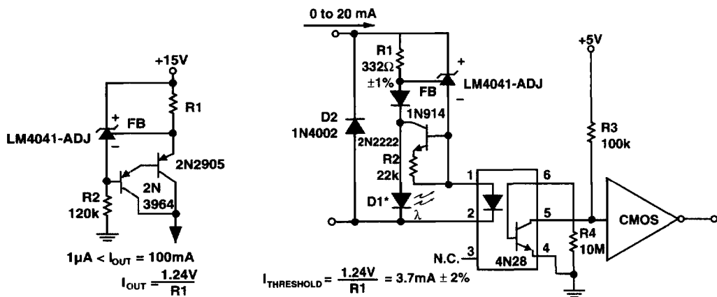
Figure 10. Current Source
