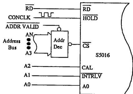
Figure 4a. Conversions Asynchronous to Master Clock
