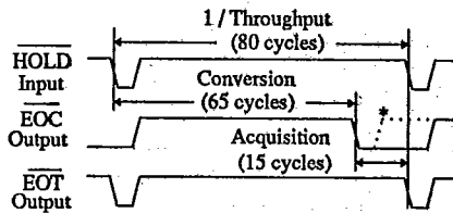
Figure 5b. Synchronous (Loopback) Mode
