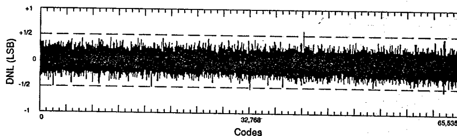
Figure 13. CS5016 Differential Nonlinearity Plot
