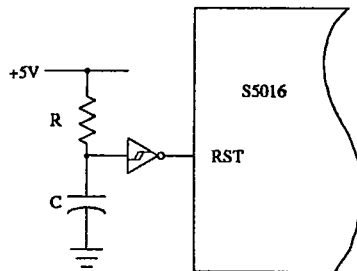
Figure 6. Power-On Reset Circuit
