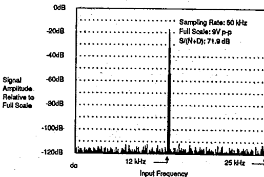
Figure 20. FFT Plot with 12 kHz -20 dB Input
