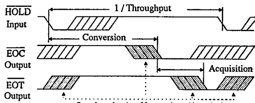
Figure 5a. Asynchronous Sampling (External Clock)
