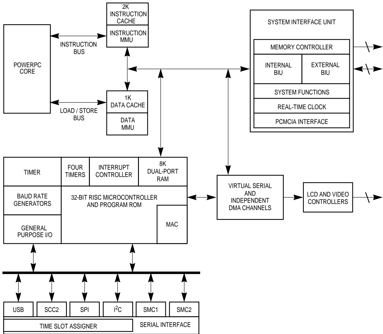
MPC823 Block Diagram
