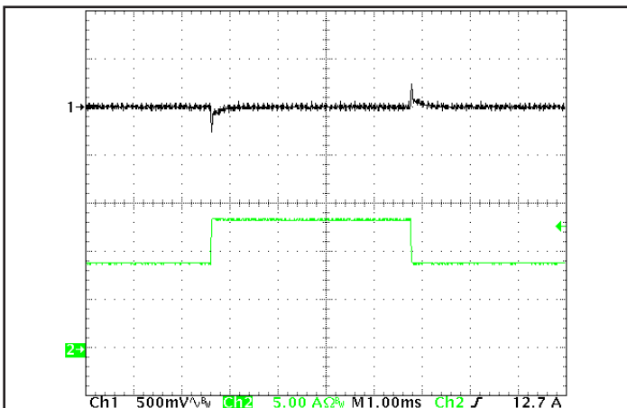
Figure 5: Output voltage response to step-change in load current (50%-75%-50% of Iout(max); dl/dt = 0.1A/us). Load cap: 15µF tantalum cap and 1µF ceramic cap. Ch 1: Vout, Ch 2: Iout.
