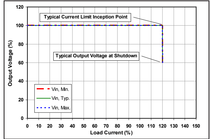
Common Figure 2: Output voltage vs. load current showing typical current limit inception curves and converter shutdown points.
