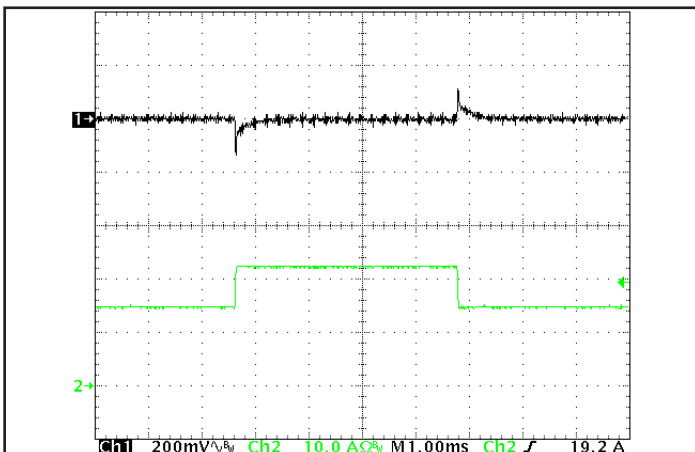
Figure 5: Output voltage response to step-change in load current (50%-75%-50% of Iout(max)); dl/dt = 0.1A/\mu s . Load cap: 15 \mu F tantalum cap and 1 \mu F ceramic cap. Ch 1: Vout, Ch 2: Iout.
