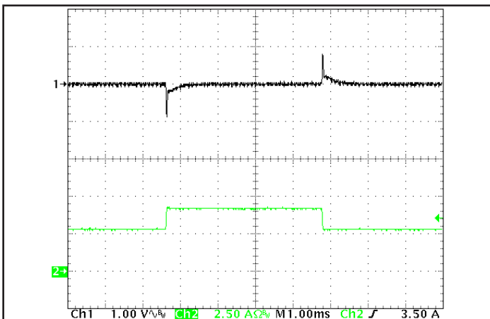
Figure 5: Output voltage response to step-change in load current (50%-75%-50% of I out (max); dl/dt = 0.1A/μs). Load cap: 1μF ceramic cap. Ch 1: V out , Ch 2: I out .
