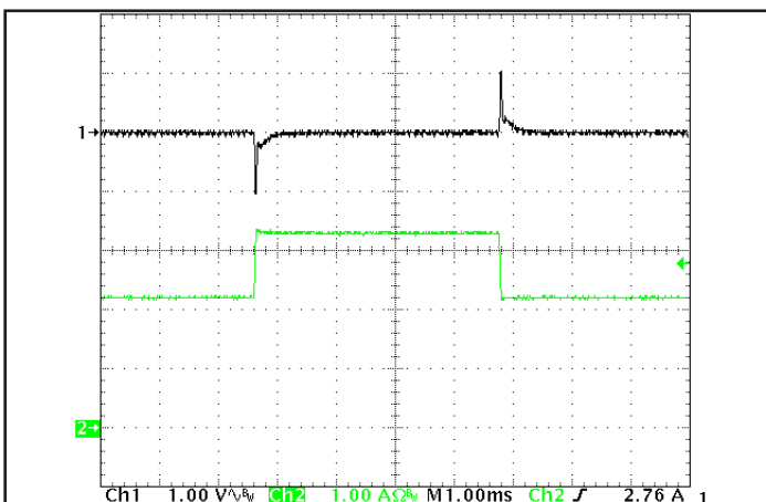
Figure 5: Output voltage response to step-change in load current (50%-75%-50% of Iout(max); dl/dt = 0.1A/us). Load cap: 1uF ceramic cap. Ch 1: Vout, Ch 2: Iout.
