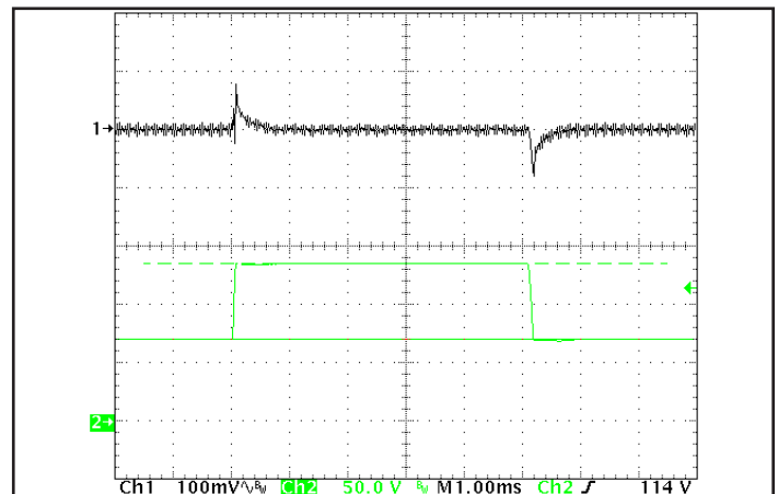
Figure 6: Output voltage response to step-change in input voltage (nominal to maximum), at full load current. Load cap: 15 \mu F tantalum capacitor and 1 \mu F ceramic cap. Ch 1: Vout, Ch 2: Vin.
