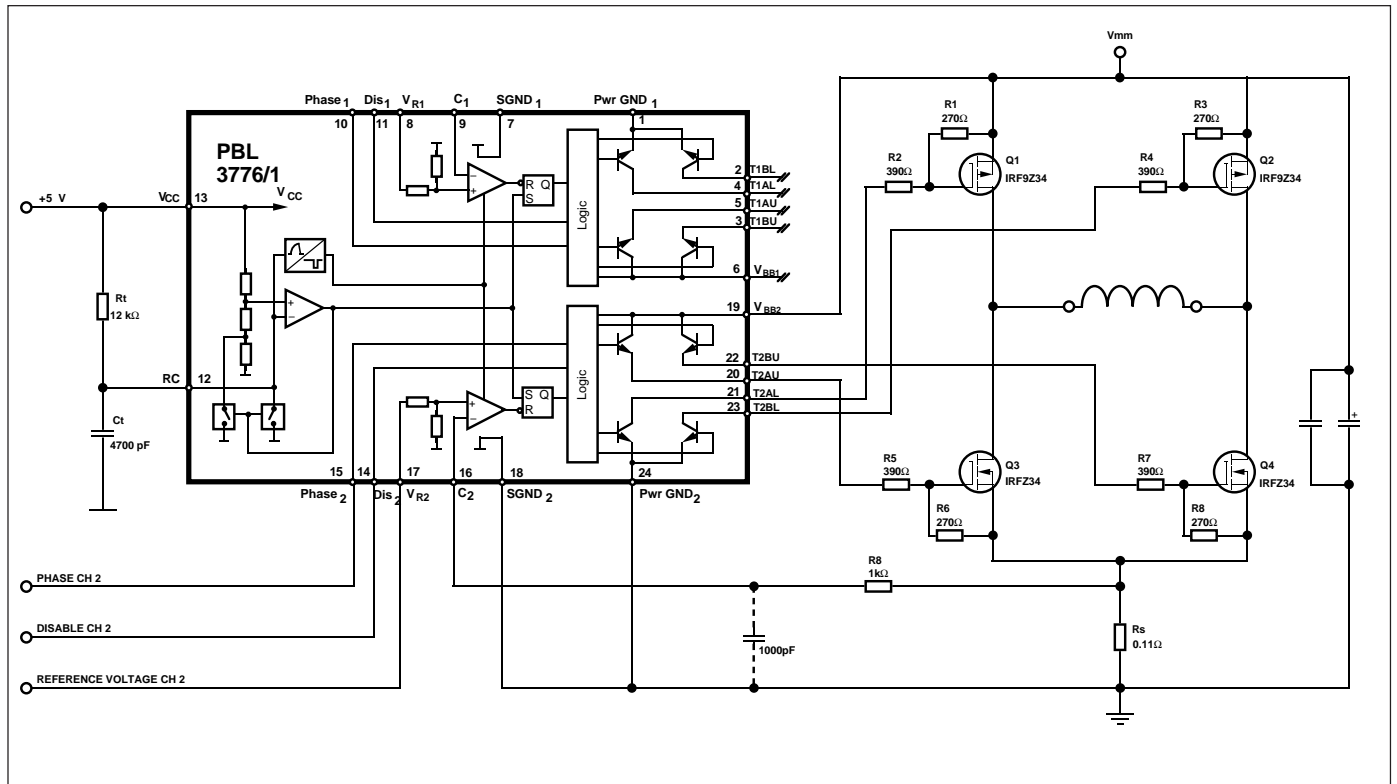
Figure 5. Typical 5 A stepper motor driver application with PBL 3776/1. One channel shown.
