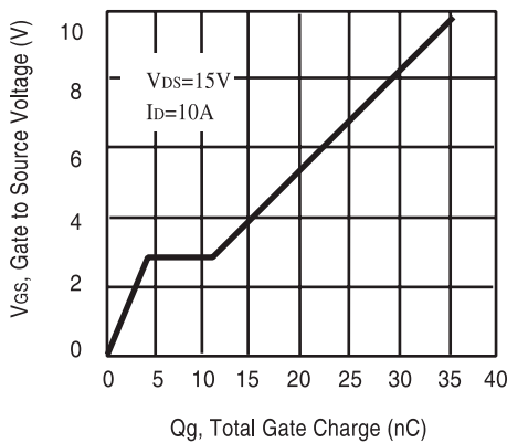
Figure 9. Gate Charge
