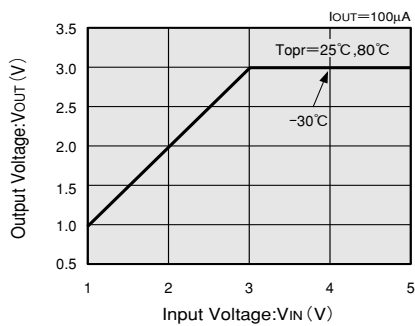
XC62RP3002 (3V)
