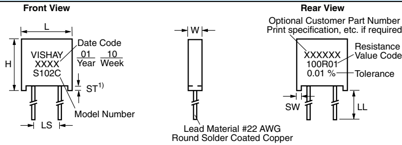
FIGURE 2 - STANDARD IMPRINTING AND DIMENSIONS
