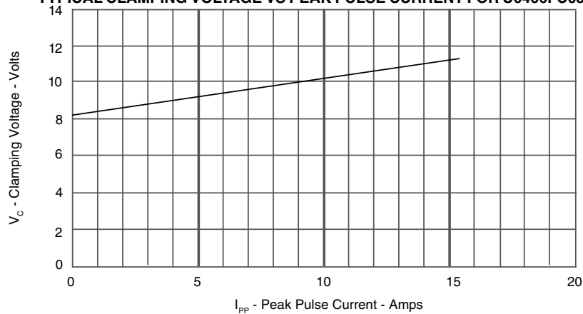
FIGURE 5 TYPICAL CLAMPING VOLTAGE VS PEAK PULSE CURRENT FOR U0406FC05C
