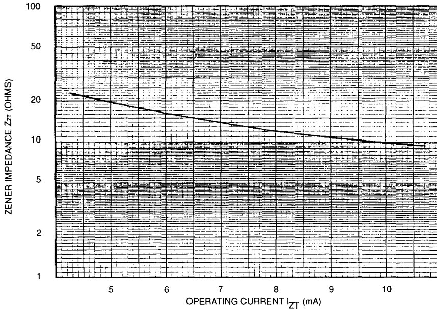
FIGURE 4 ZENER IMPEDANCE VS. OPERATING CURRENT
