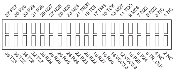
Figure 8. Debug Mictor Connector - J20
