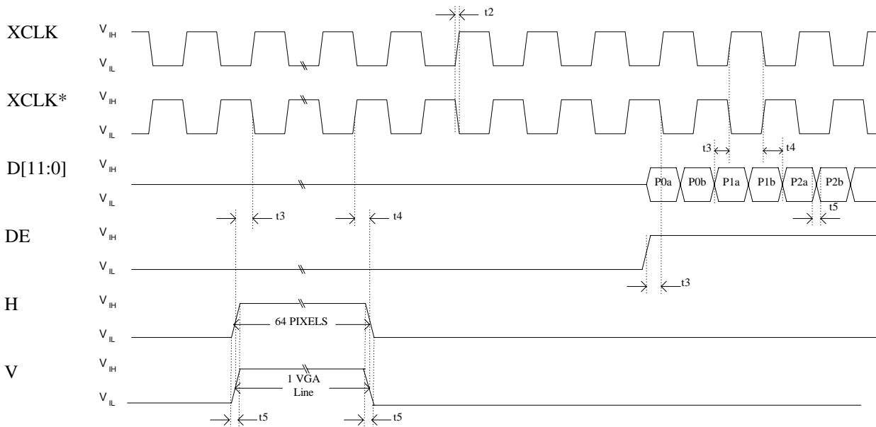
Figure 18: Timing for Clock - Slave, Sync - Slave Mode
