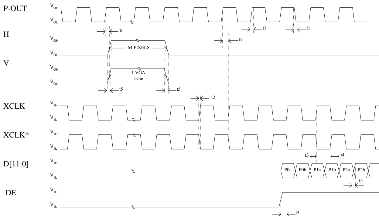
Figure 20: Clock - Master, Sync - Master Mode
