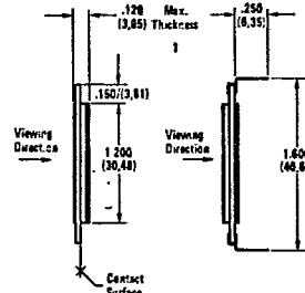
PINLESS CONFIGURATION
