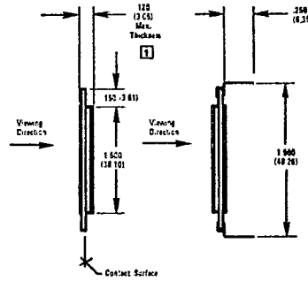
PINNED CONFIGURATION
