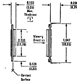
PINLESS CONFIGURATION
