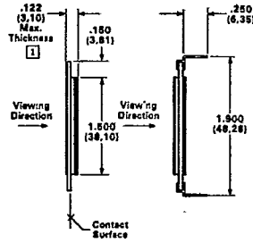
PINLESS CONFIGURATION
