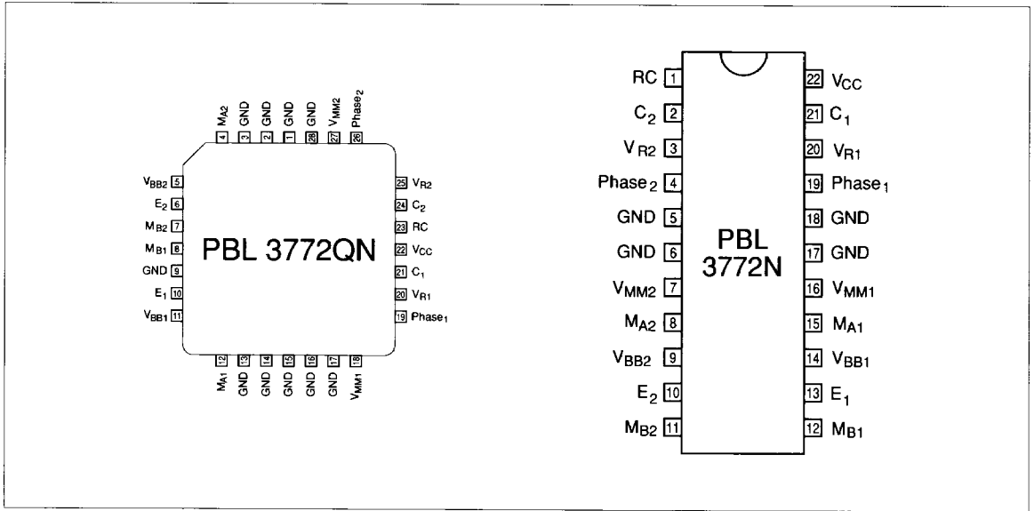
Figure 4. Pin configuration.
