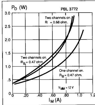
Figure 8. Power dissipation vs. motor current. T_a = 25^\circ \text{C} .
