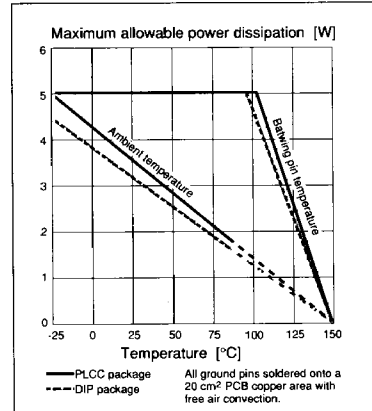
Figure 10. Maximum allowable power dissipation vs. temperature.
