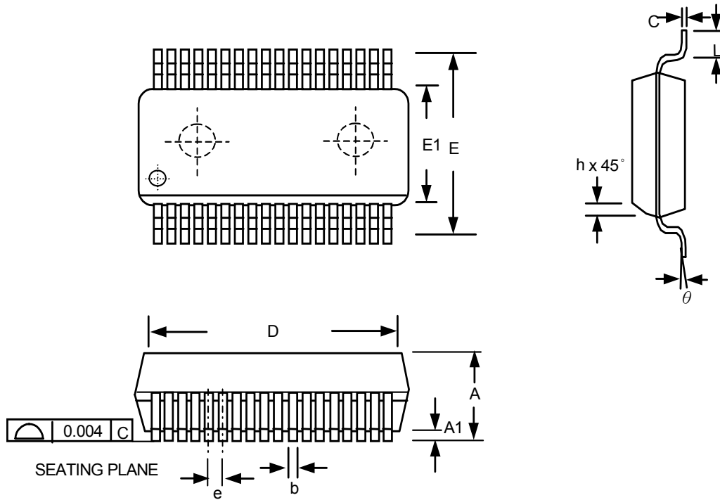
SSOP-36 Package
