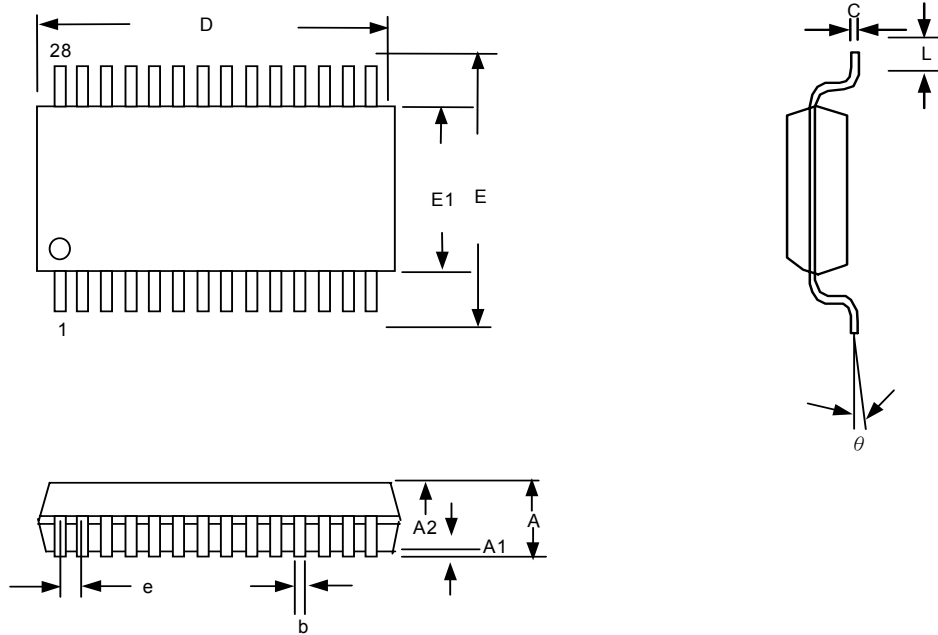
TSSOP-28 Package
